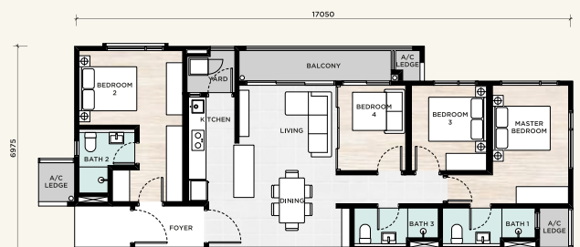
TYPE D 1,236 SQ. FT. | 4 3 DUAL-KEY
